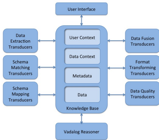
Figure 1: VADA Architecture.
